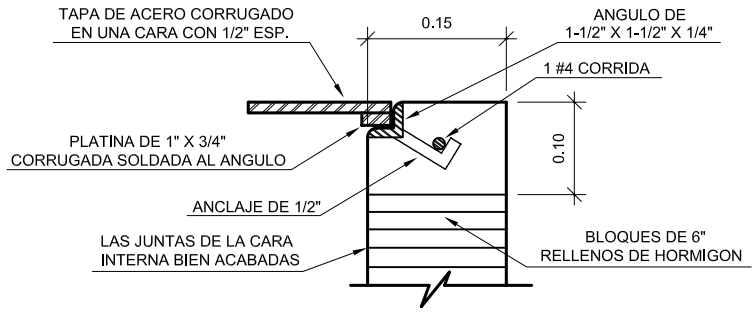
DETALLE "E"
